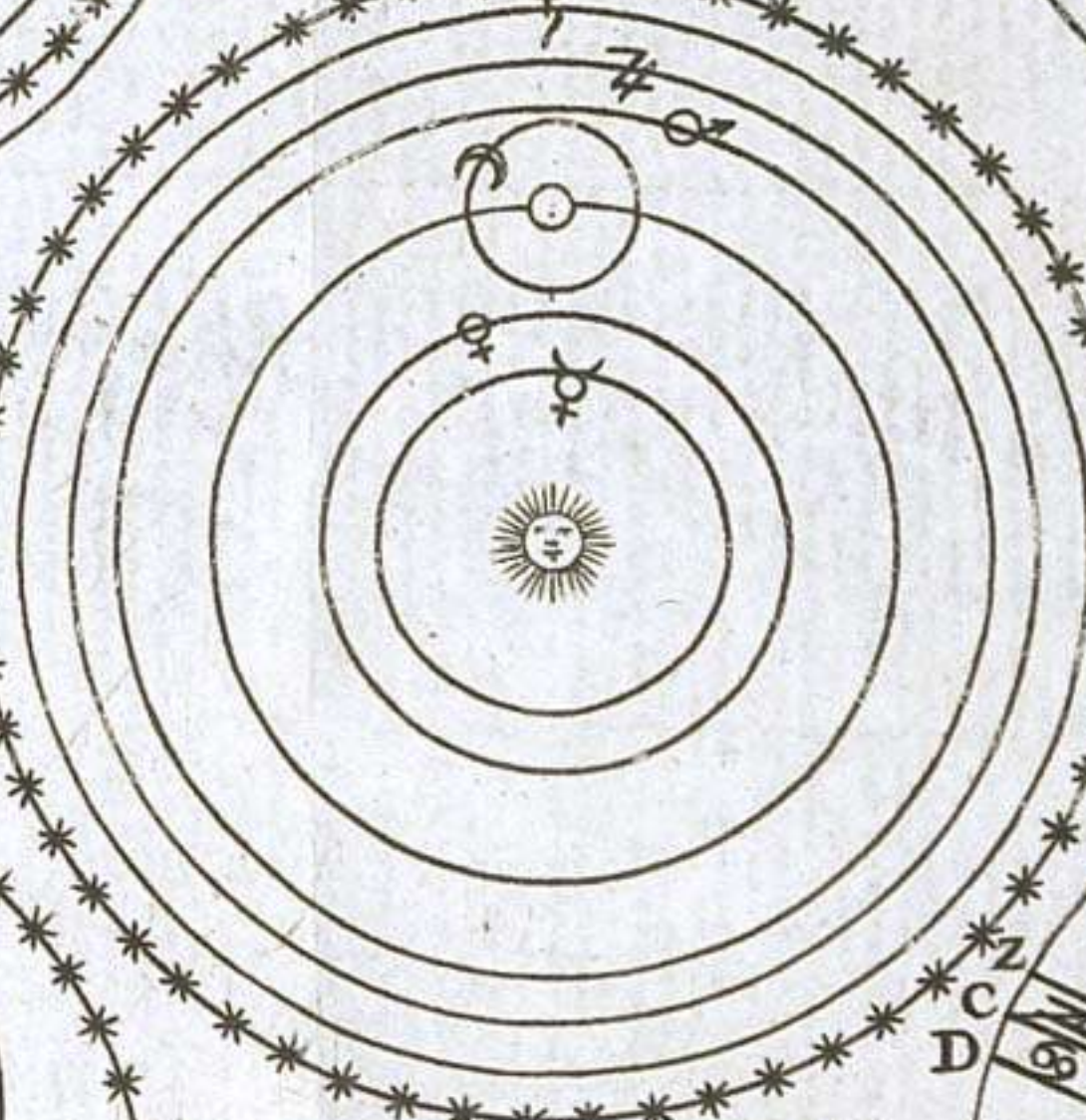
3. Systhema Copernicanum.
