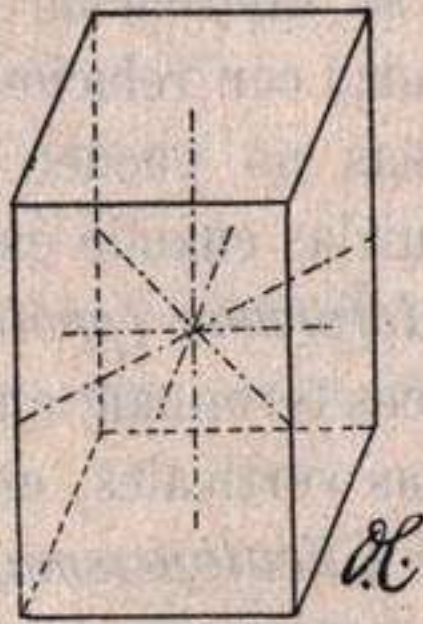
Fig. 106. — Prisma tetragonal.
