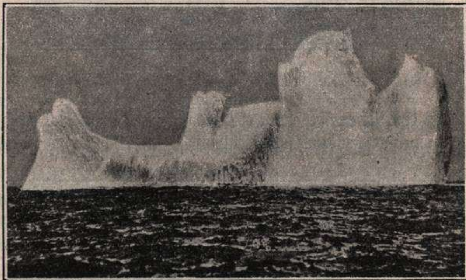
Fig. 350.—Un iceberg.
