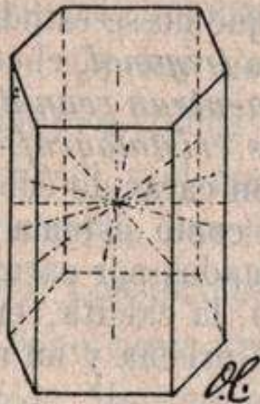
Fig. 102.—Prisma exagonal.
