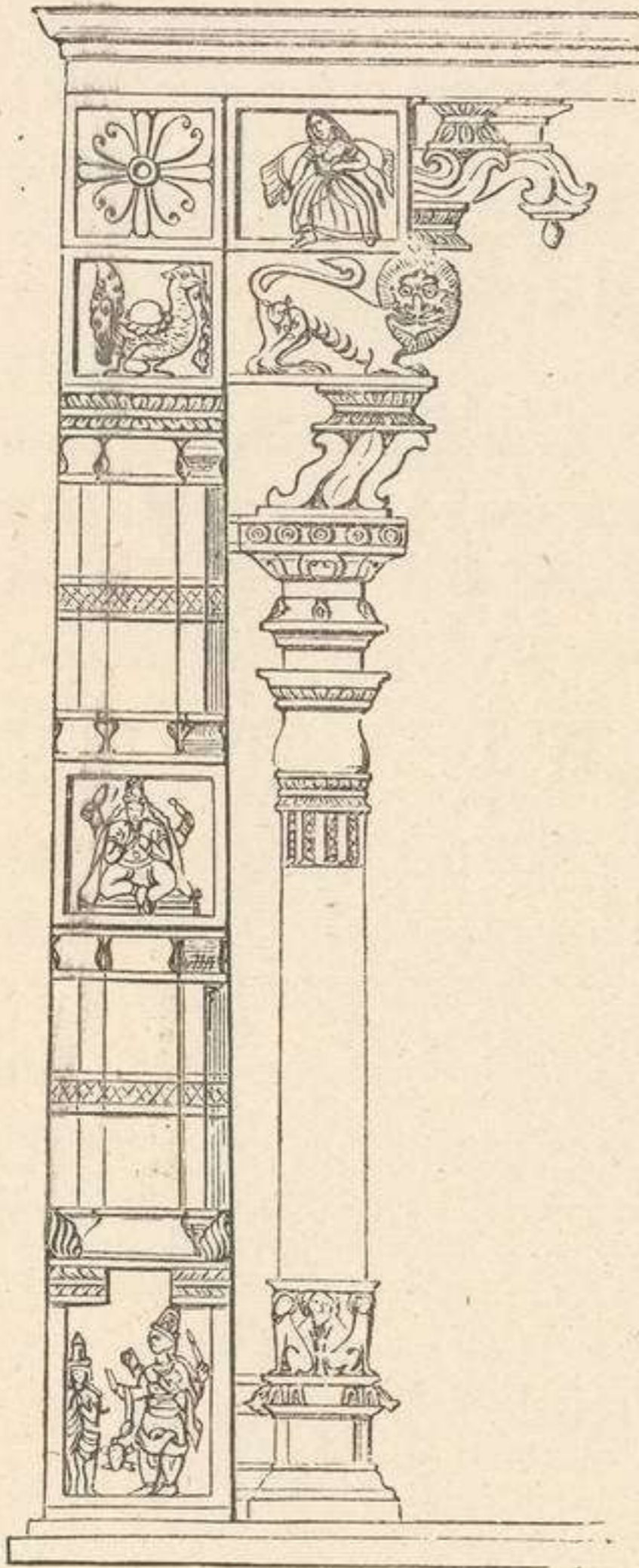
Fig. 328.—Pillar and Bracket, Doorway of a Pagoda.
