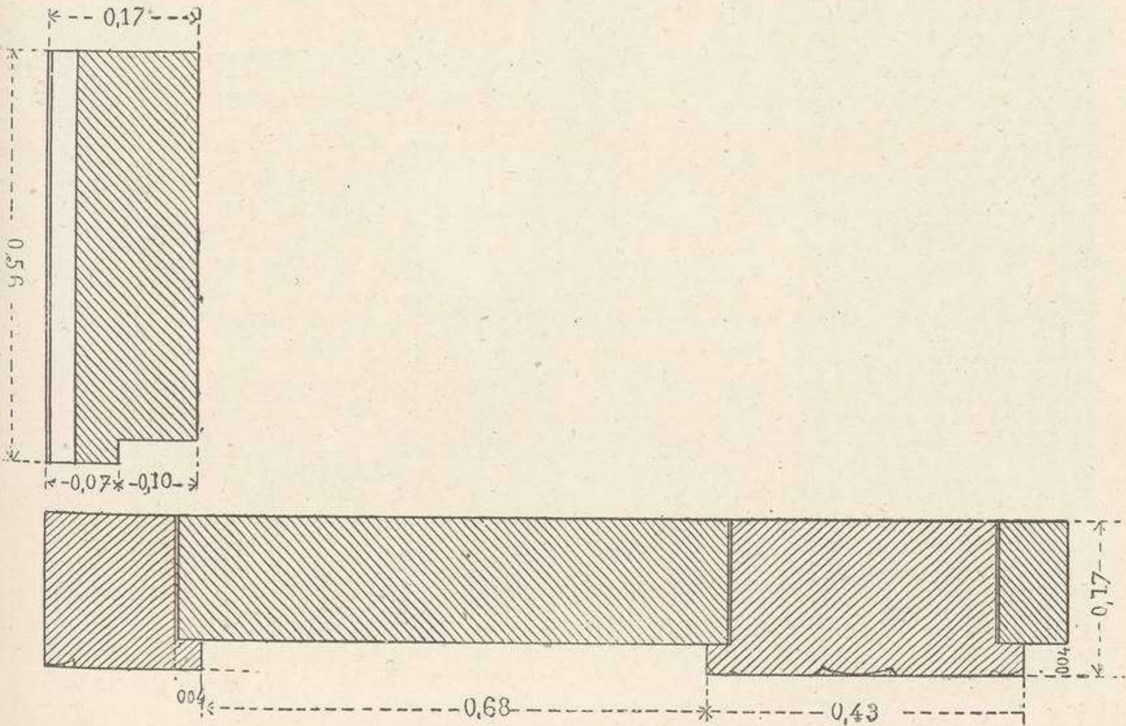
Fig. 279.—Plan of Fig. 278, Alabaster Frieze. (P. & C.)
