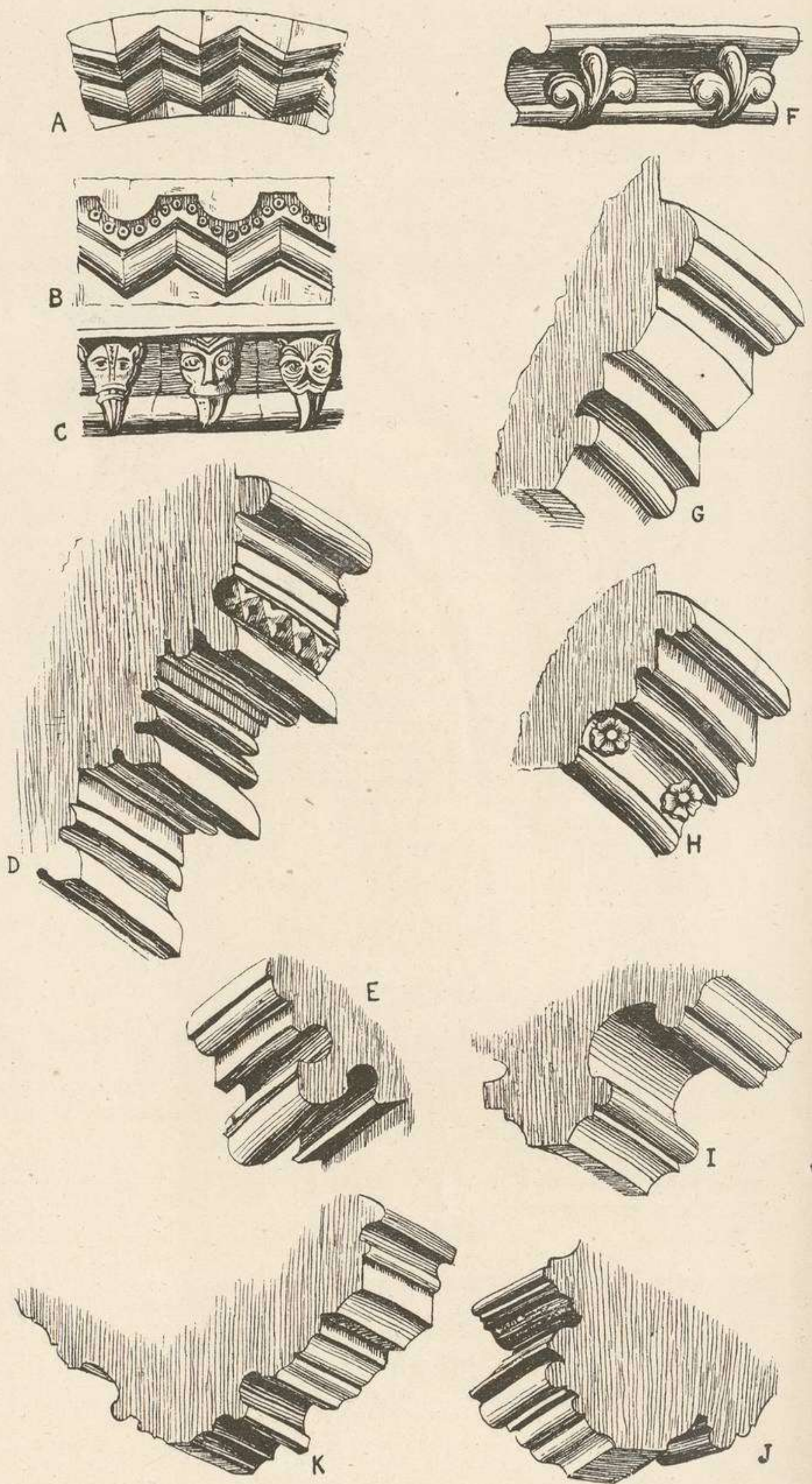
Fig. 401.— Norman and Gothic Mouldings.
