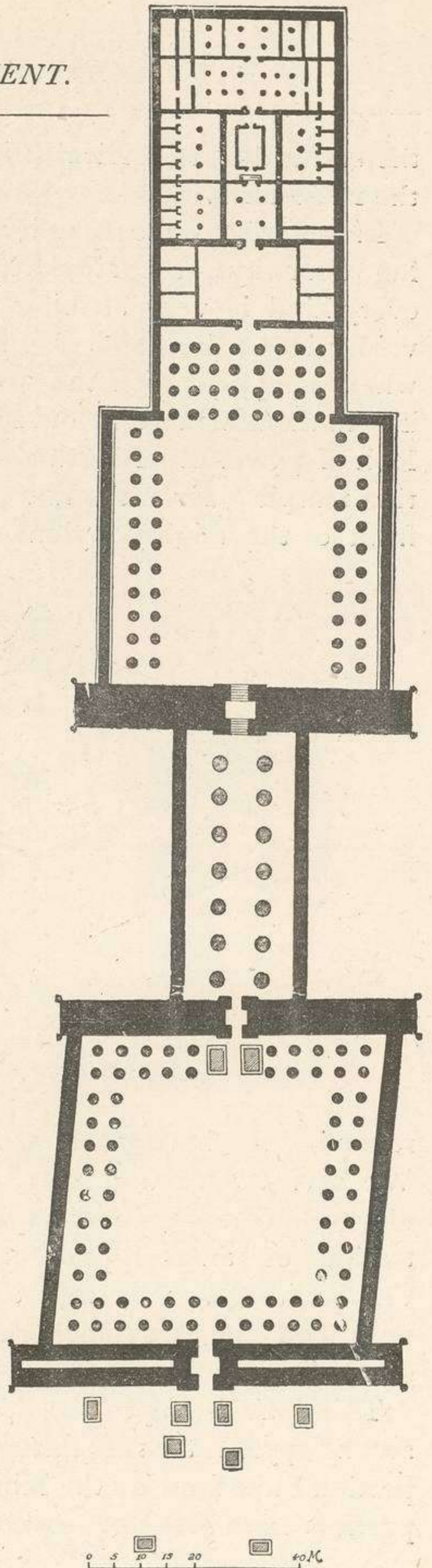
Fig. 106.—Plan of the Temple of Luxor. (P. & C.)
