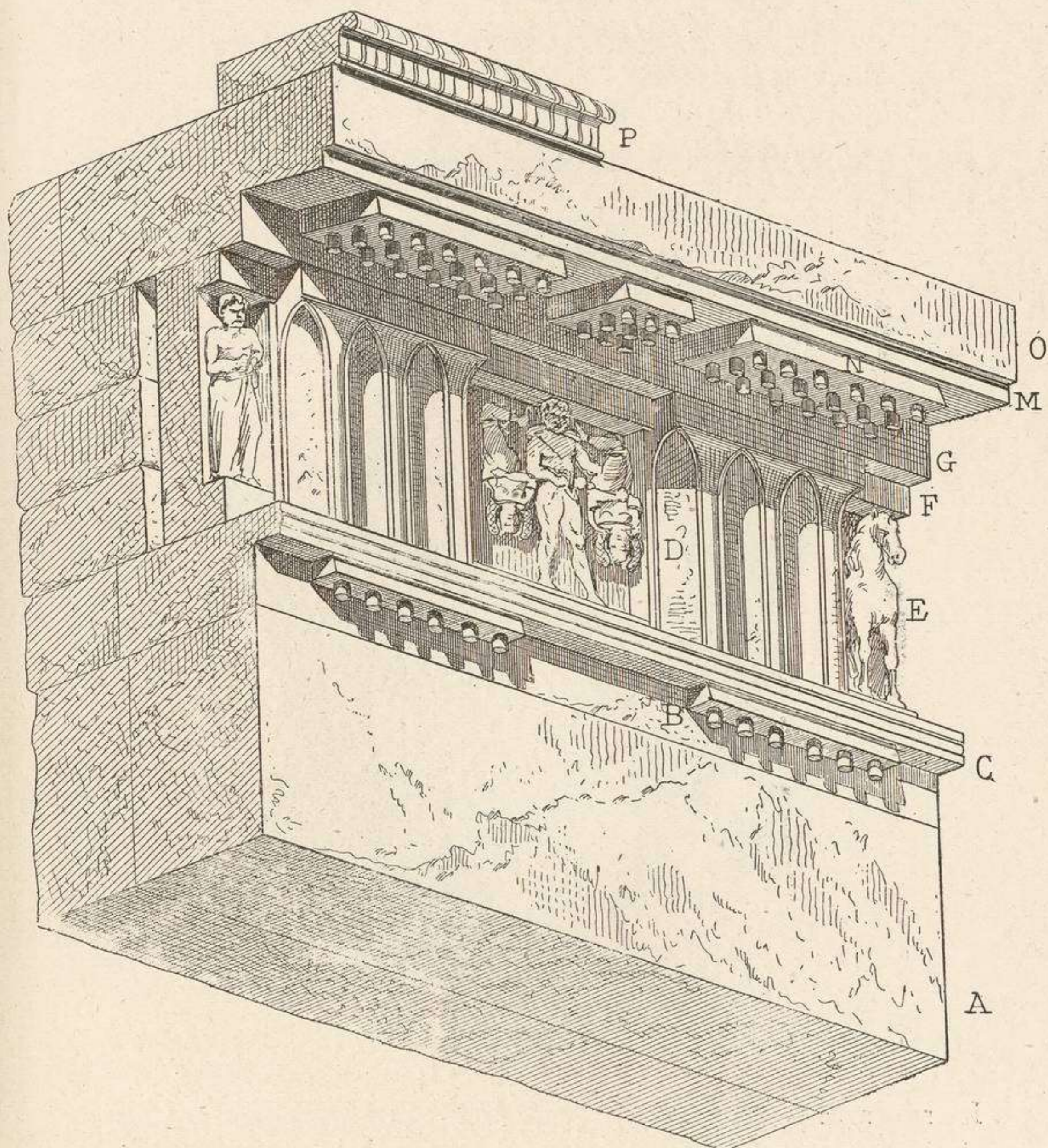
Fig. 284.—Entablature of C. Selinous Temple. (P. & C.)
